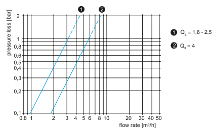
Typical pressure loss curve
