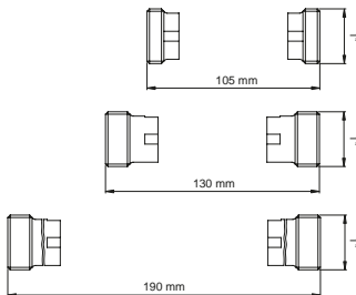
Connection thread 1"
